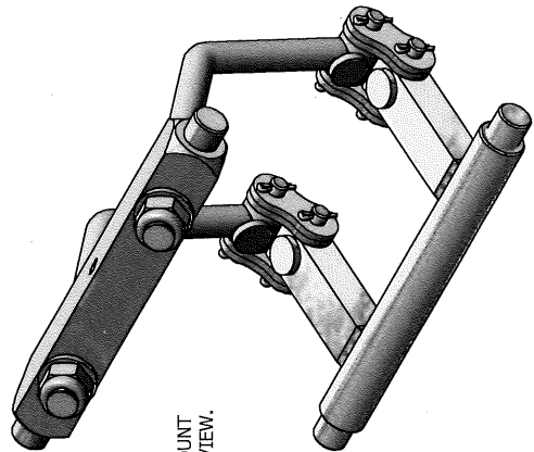
ITEMS 9 & 10 ARE THE DIFFERENT PARTS REQUIRED FOR 100mm x 100mm BOX. ALL OTHER PARTS ARE COMMON.
