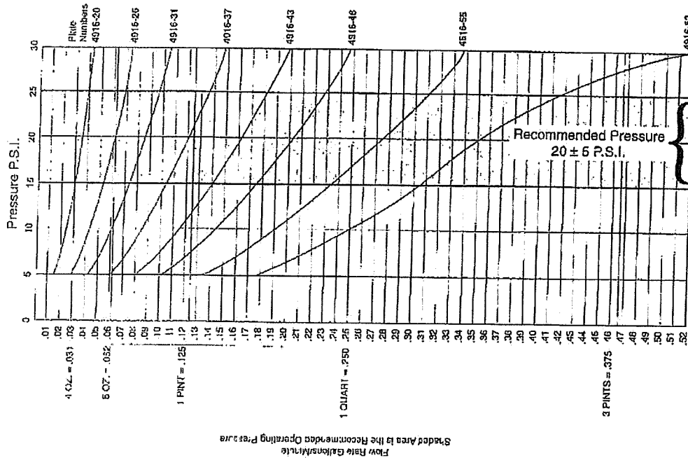
Graph for Determining the Flow Rate of Different Orifice Plates 4916-83
