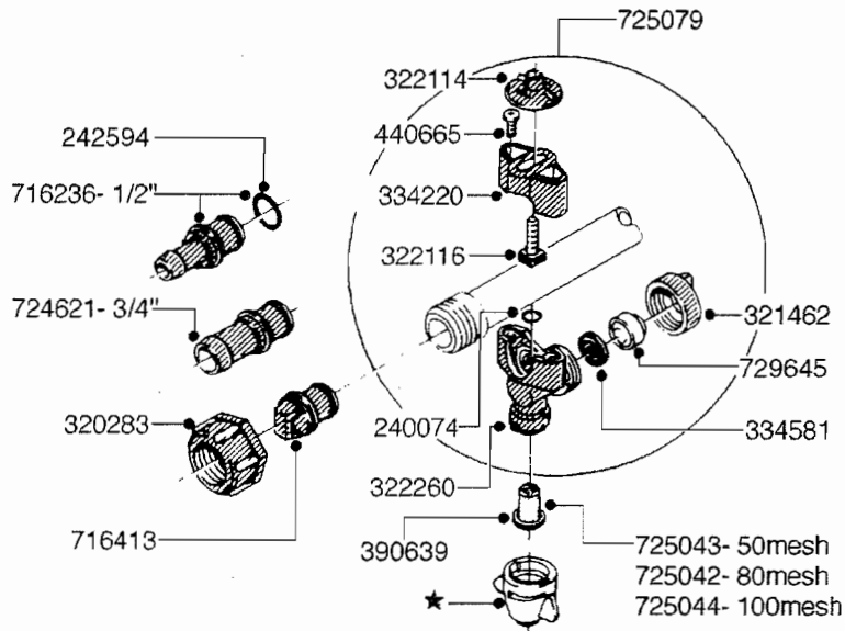
SINGLE NOZZLE BODY
