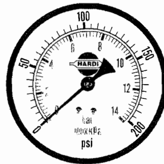
28014403 200 psi (14 bar) STAINLESS 4" GAUGE
