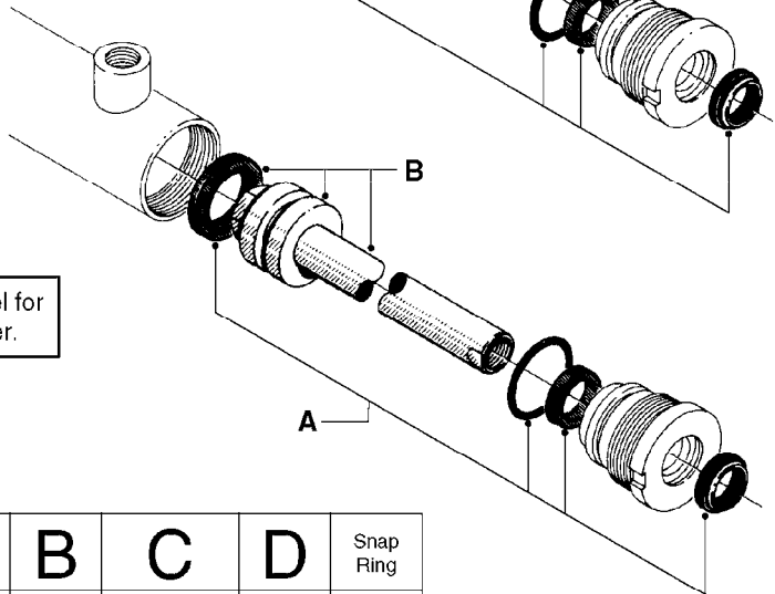
SINGLE-ACTING CYLINDER
