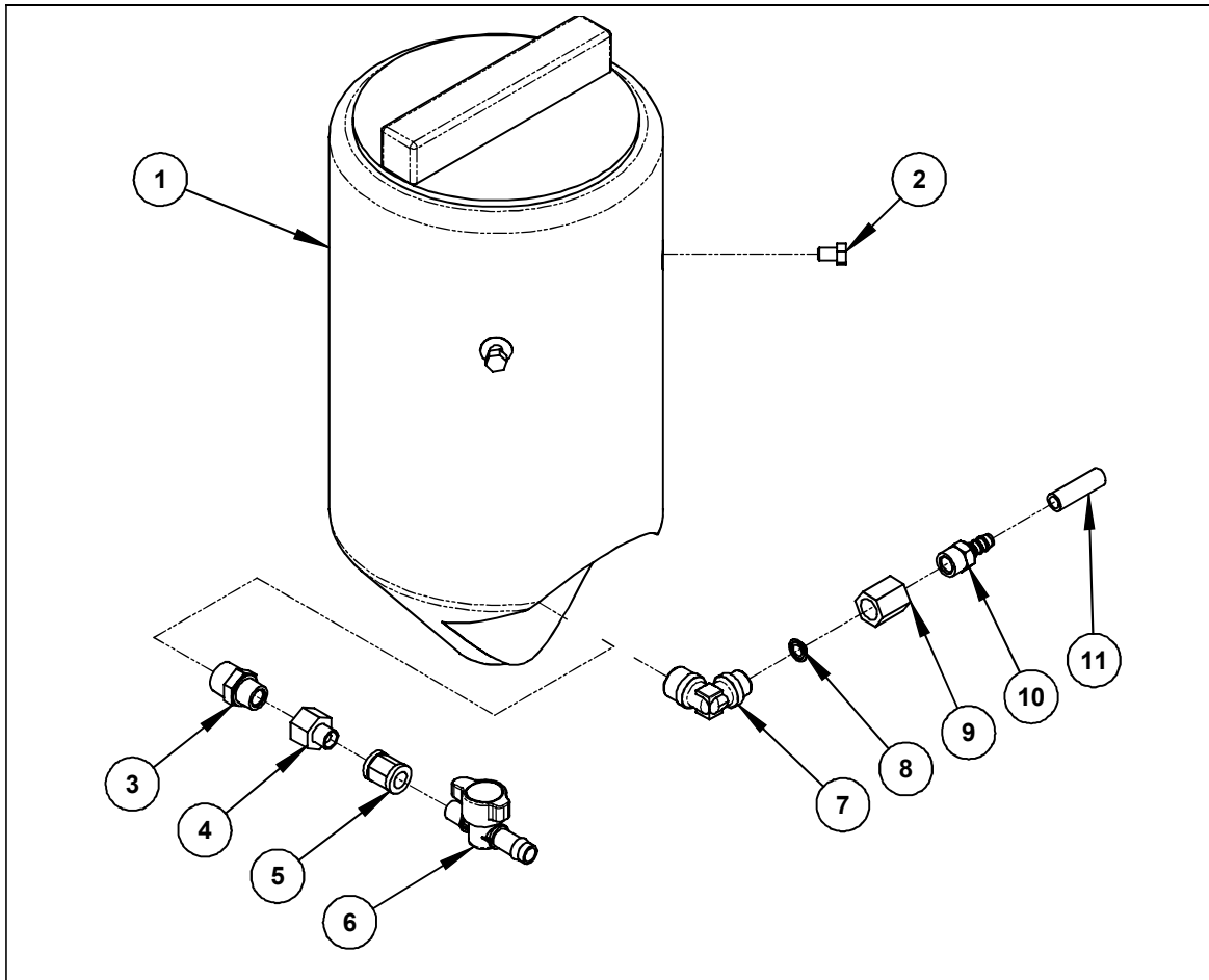
Figure 8 – Rinse and Hand-Wash Tank Components
