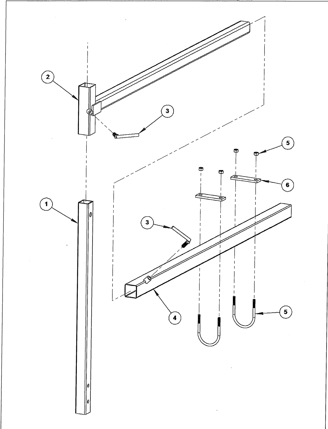
Figure 15 – Mounting Assembly, Standard
